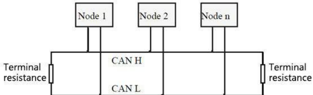
Figure 3.1 CAN-Bus network structure
