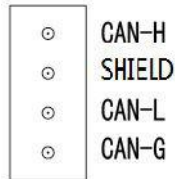
Figure 2.7 CAN bus terminal block of GCAN-PLC-511
