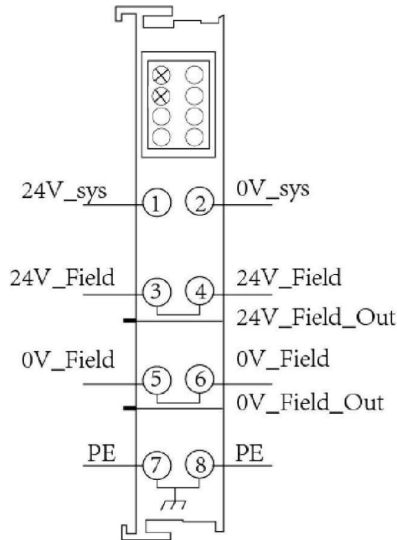
Figure 2.8 GCAN-PLC-511, Power terminal block
