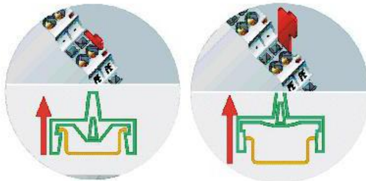
Figure 2.3 GCAN-PLC-511 self-locking mechanism
