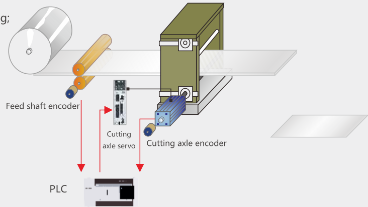
E-cam -- Flying shear function
