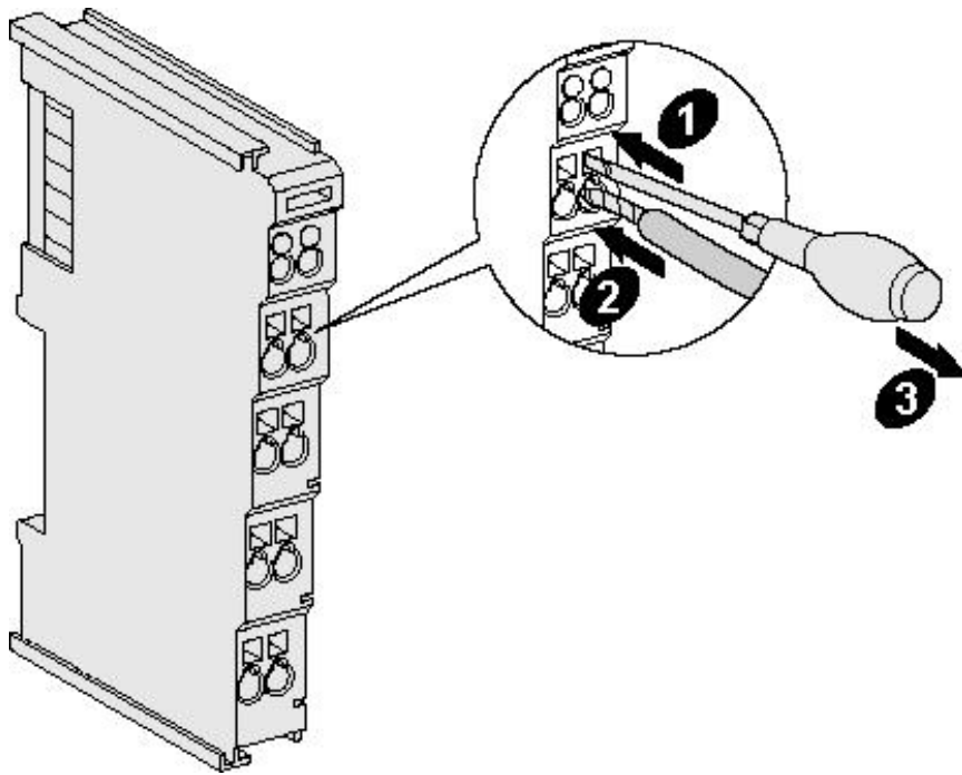
Figure 2.2 GC-3822 module installation
