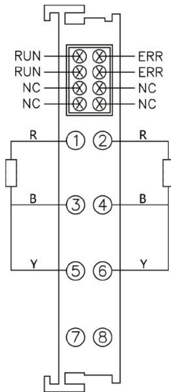
Figure 2.3 GC-3822 module terminal block
