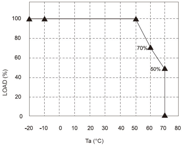
OUTPUT DERATING VS Ta
