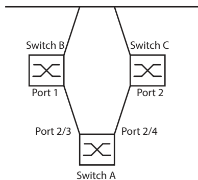
Figure 61: Link Backup example network
