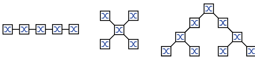
Figure 30: Network with line, star and tree topologies
