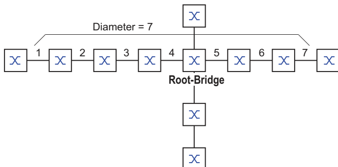
Figure 53: Definition of diameter
