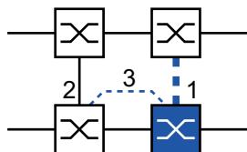
Figure 75: Two-Switch coupling with Control Line, Stand-by device 1: Coupling port 2: Partner coupling port 3: Control line
