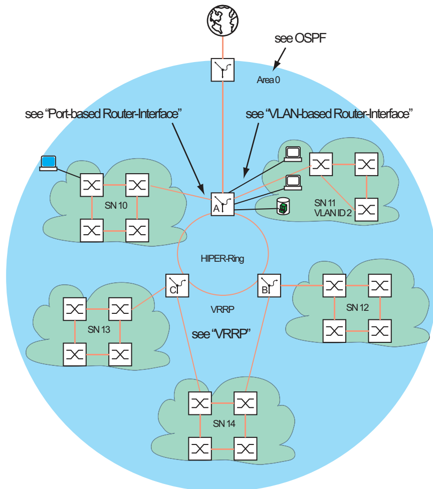
Figure 115: Network plan
