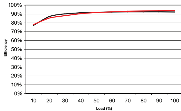
Figure 8 - AHM85PS24
