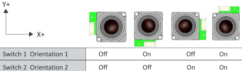
Figure.1 Mounting Orientations
