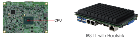
IB811 with Heatsink
