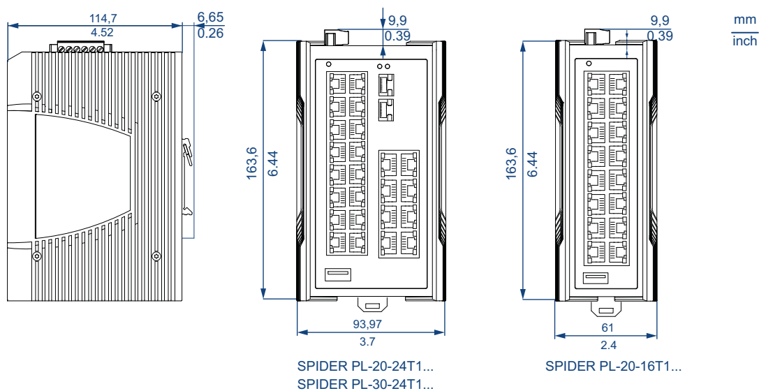
Figure 5: Dimensions of device variants SPIDER PL-20... and SPIDER PL-30...
