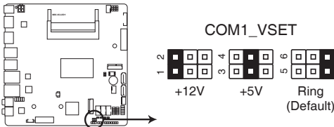
MIX-KLUD1 COM1 Ring/+5V/+12V selection
