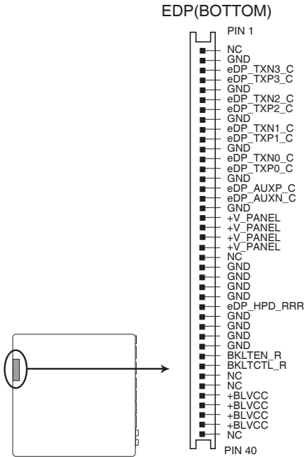
MIX-KLUD1 Embedded DisplayPort
