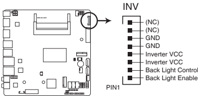
MIX-KLUD1 Inverter connector
