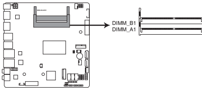
MIX-KLUD1 260-pin DDR4 SO-DIMM sockets
