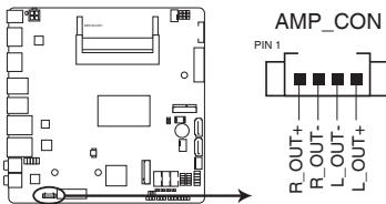
MIX-KLUD1 Audio stereo output with Amp connector
