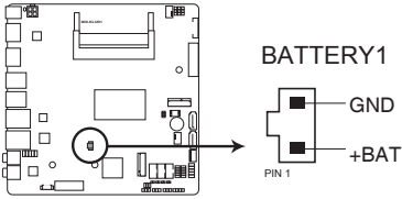
MIX-KLUD1 BATTERY connector
