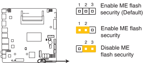
MIX-KLUD1 Intel® ME jumper
