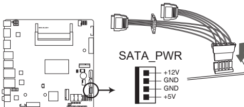
MIX-KLUD1 SATA power connector
