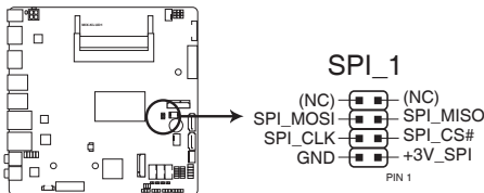
MIX-KLUD1 BIOS Programmable connector
