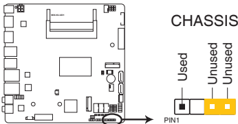
MIX-KLUD1 Chassis intrusion connector
