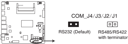
MIX-KLUD1 COM1 operating mode selection jumpers
