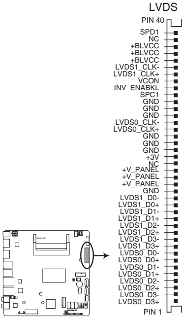
MIX-KLUD1 LVDS connector
