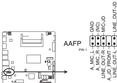
MIX-KLUD1 Front panel audio connector
