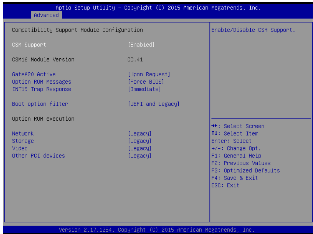
Figure 3.30 CSM Configuration
