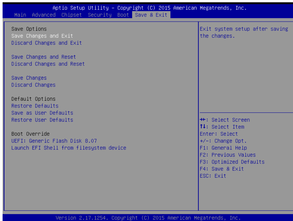
Figure 3.43 Save & Exit
