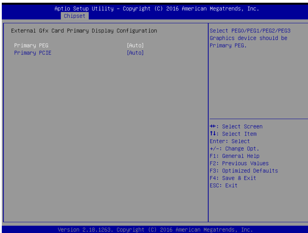
Figure 3.34 Graphics Configuration
