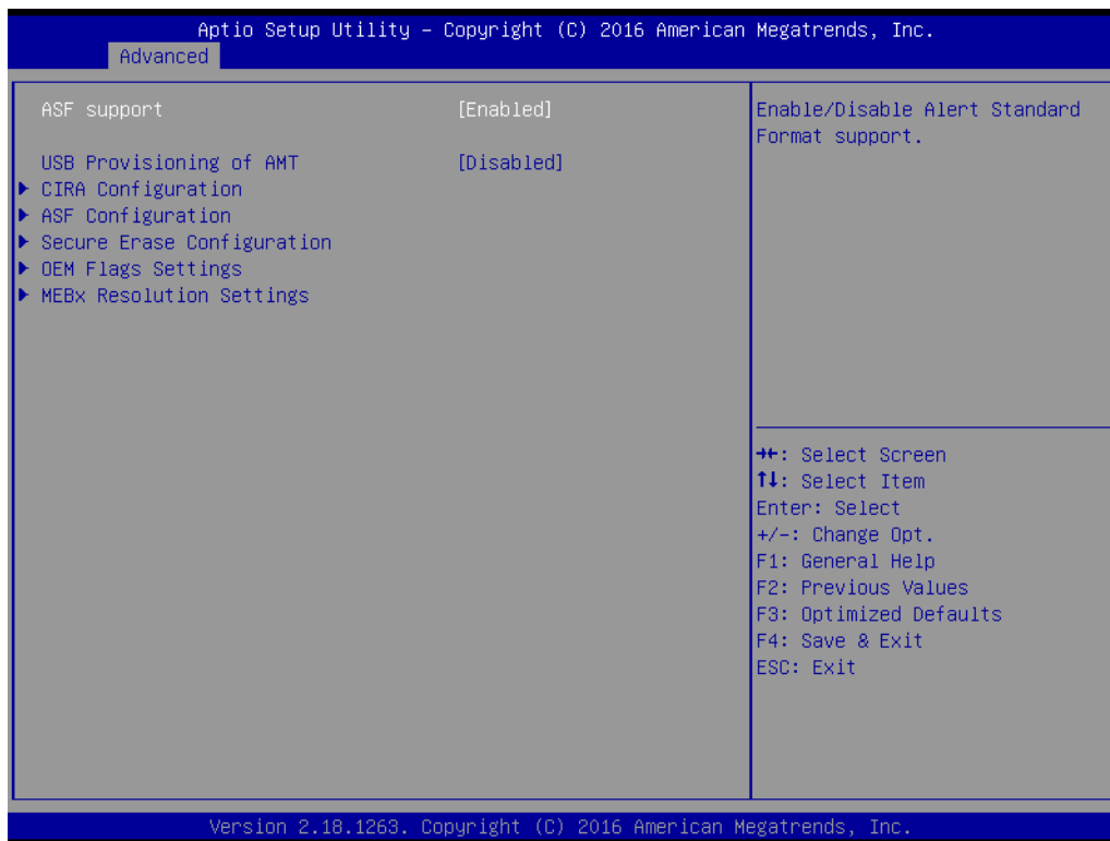
Figure 3.7 AMT Configuration
